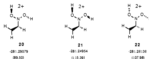
Figure 8. 4-31G single-point calculations of triply rotated conformations. Total energies (au) and rotational energy differences (in parentheses; kcal/mol) from 17.
