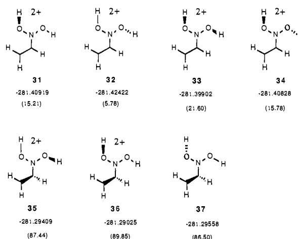
Figure 12. 4-31G single-point calculations of rotated conformations. Total energies (au) and rotational energy differences (in parentheses; kcal/mol) from 17 .
