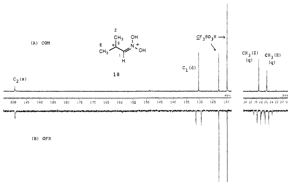
Figure 4. 100-MHz ^{13}\text{C} NMR spectrum of 1-nitro-2-methyl-1-propene in TFSA at -20\text{ }^\circ\text{C} : (A) complete proton-decoupled spectrum; (B) off-resonance proton-decoupled spectrum.
